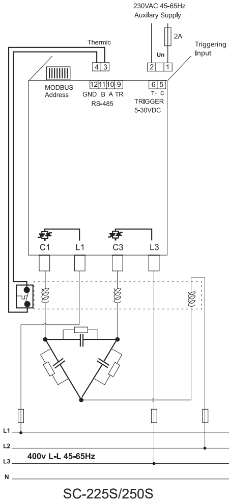
Connection Diagram
