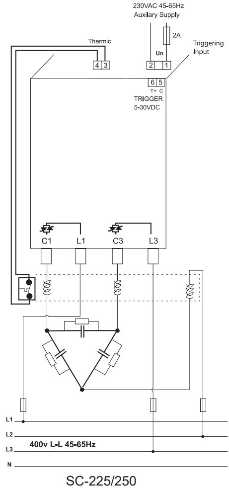
Connection Diagram
